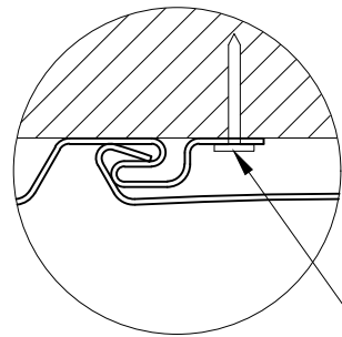
DETAIL "J"
