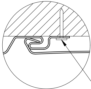
DETAIL "J"
